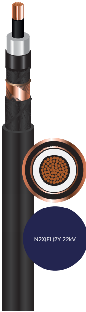
N2XCH IEC 60502-1 XLPE CWS FRNC 0.6/1kV CABLE
